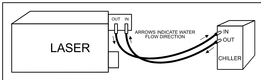
Chiller Connections
